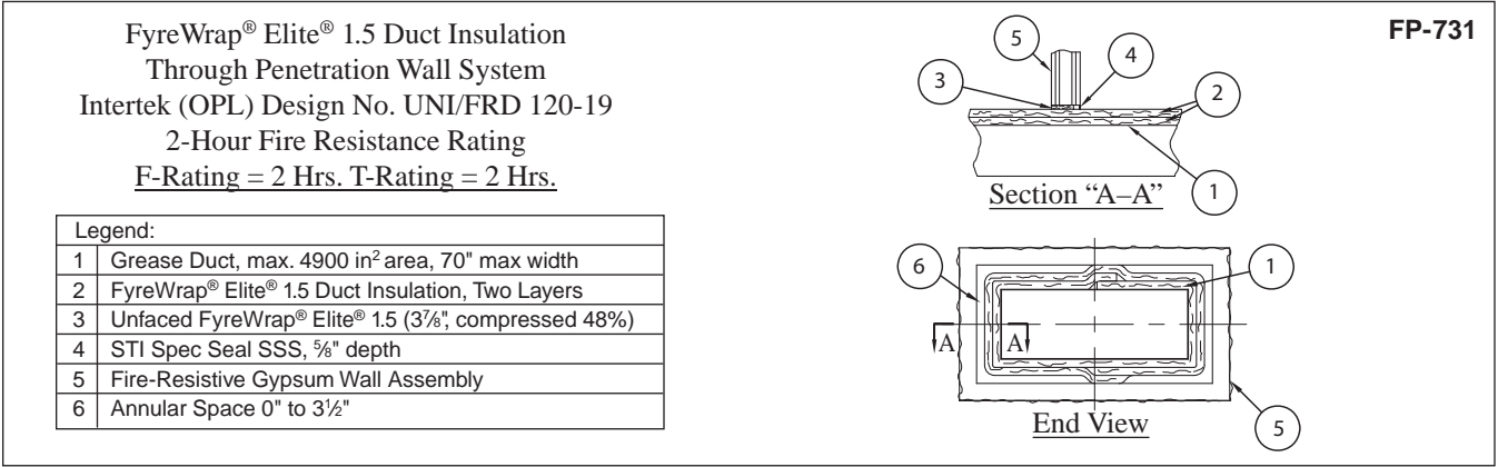
Figure 5. Firestop Installation
