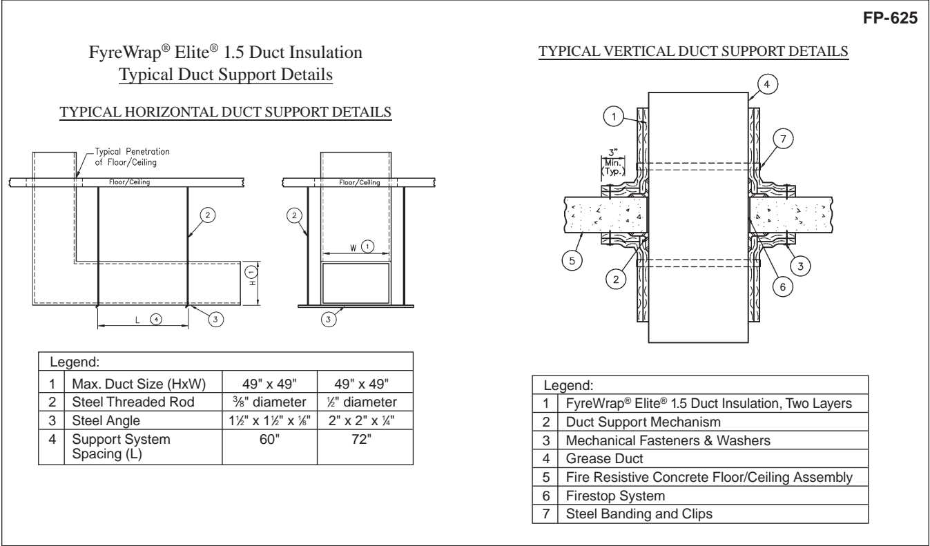
Figure 4. Firestop Installation
