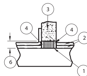
Section "A-A" Option 5
