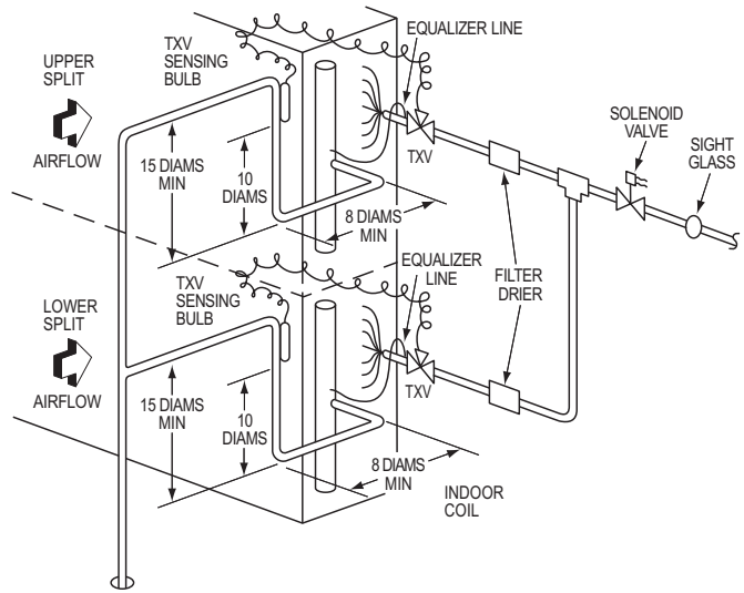
Dual Circuit Coil Piping Configuration - FAS120-300, FHS120-240 For single compressor condensing units
