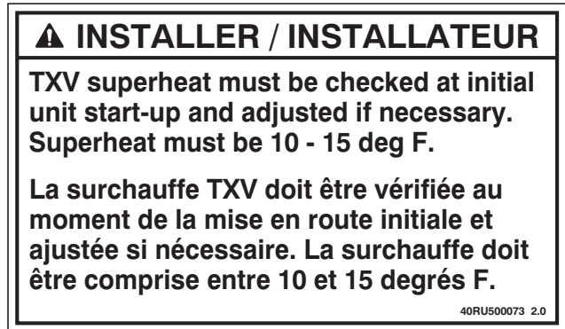
Fig. 21 - Label, TXV Adjustment
