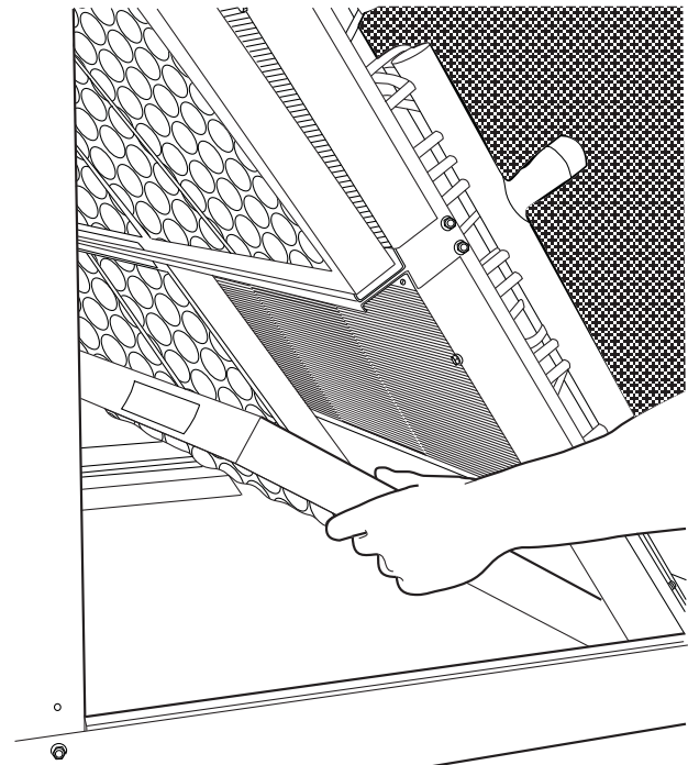
Fig. 28 - Filter Removal/Replacement
