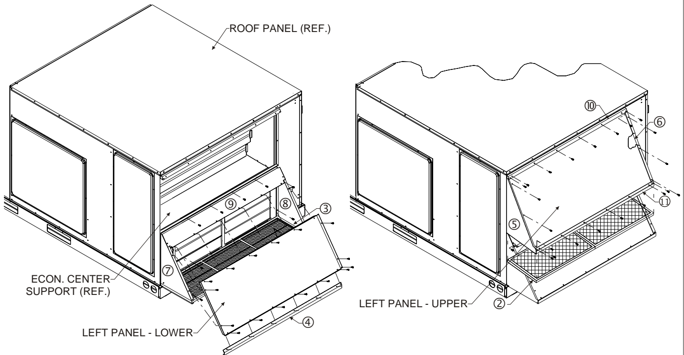
FIGURE 3 (-)XRD-PDCM3 Shown - (-)XRD-SDCM3 Similar (See Table 1 for identification of parts)
