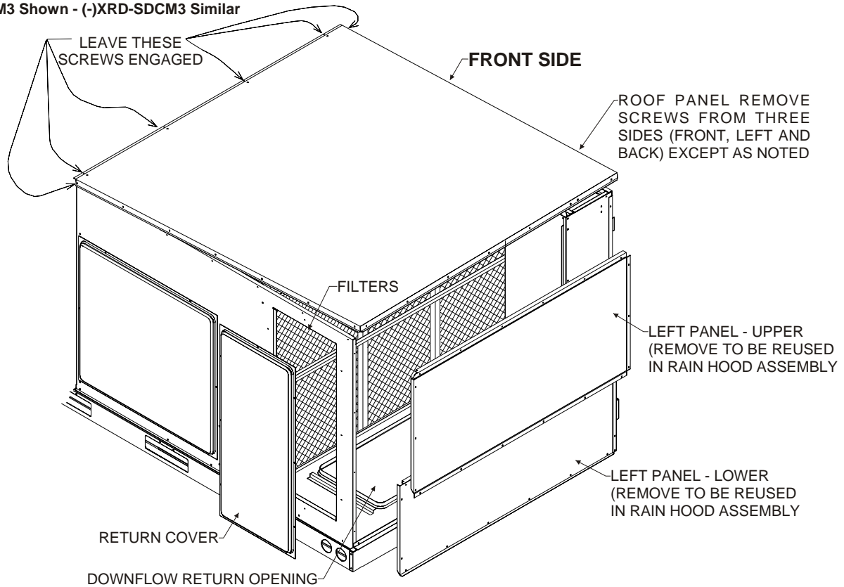
FIGURE 1 (-)XRD-PDCM3 Shown - (-)XRD-SDCM3 Similar
