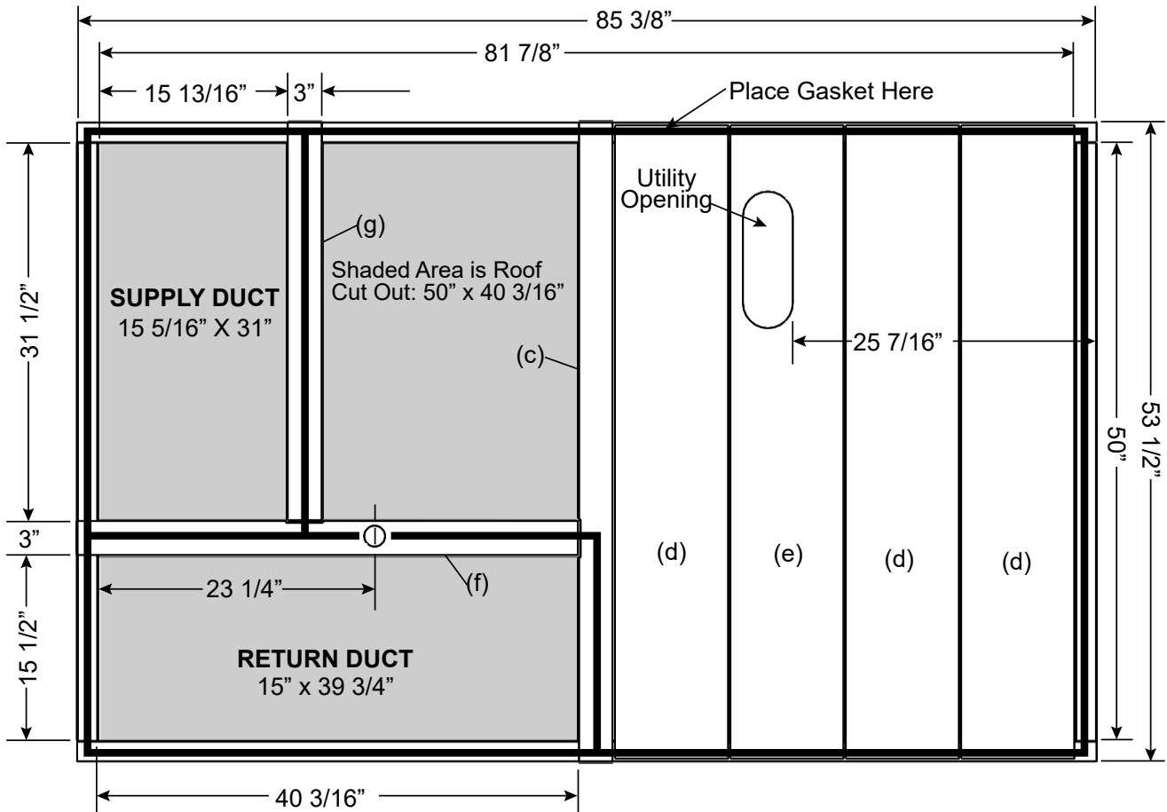
Figure 5 - Top View
