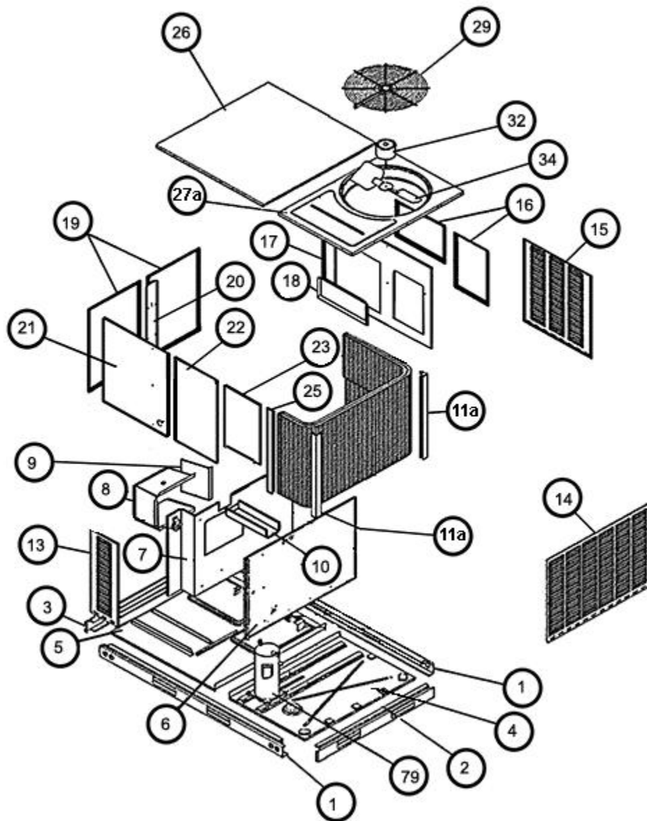
Exploded View 036-060
