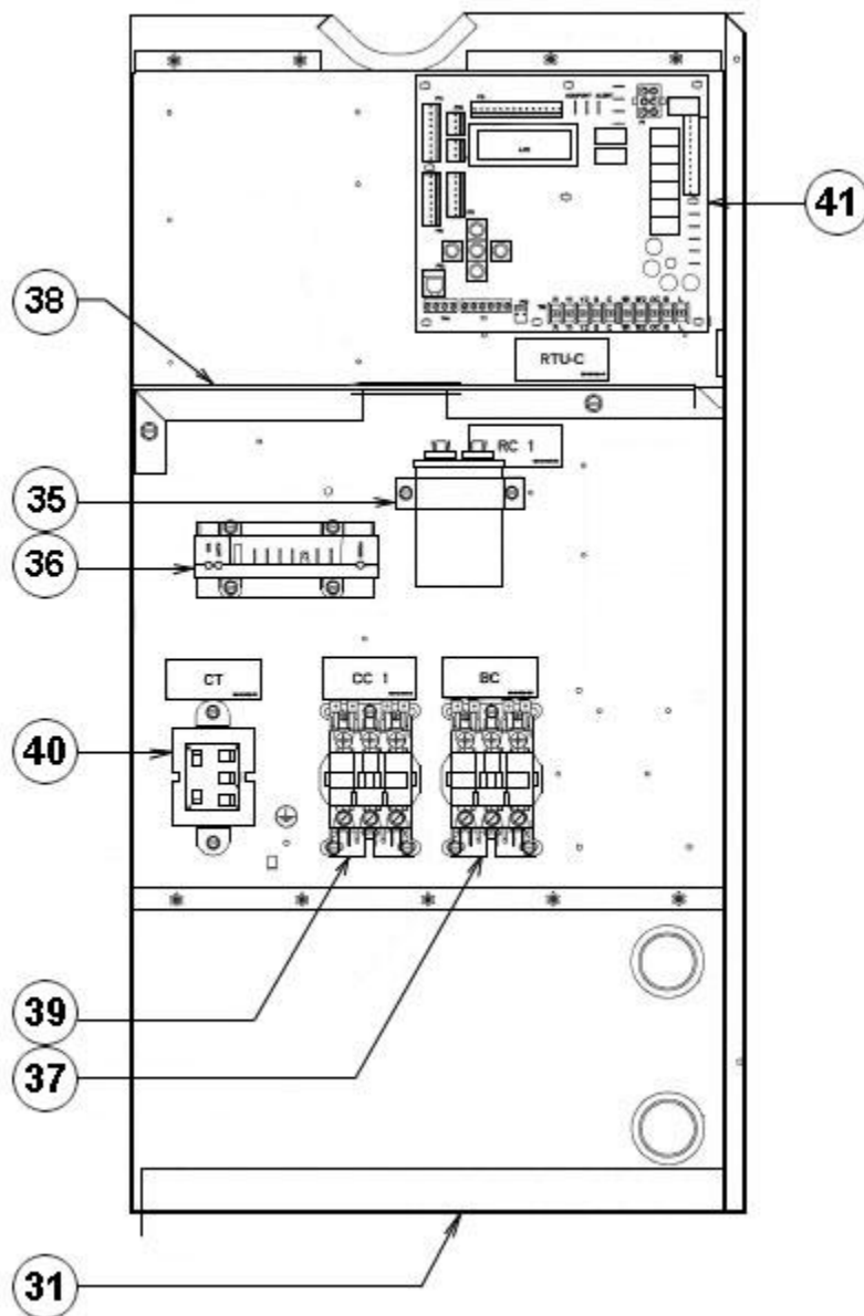
Control Box 036-060
