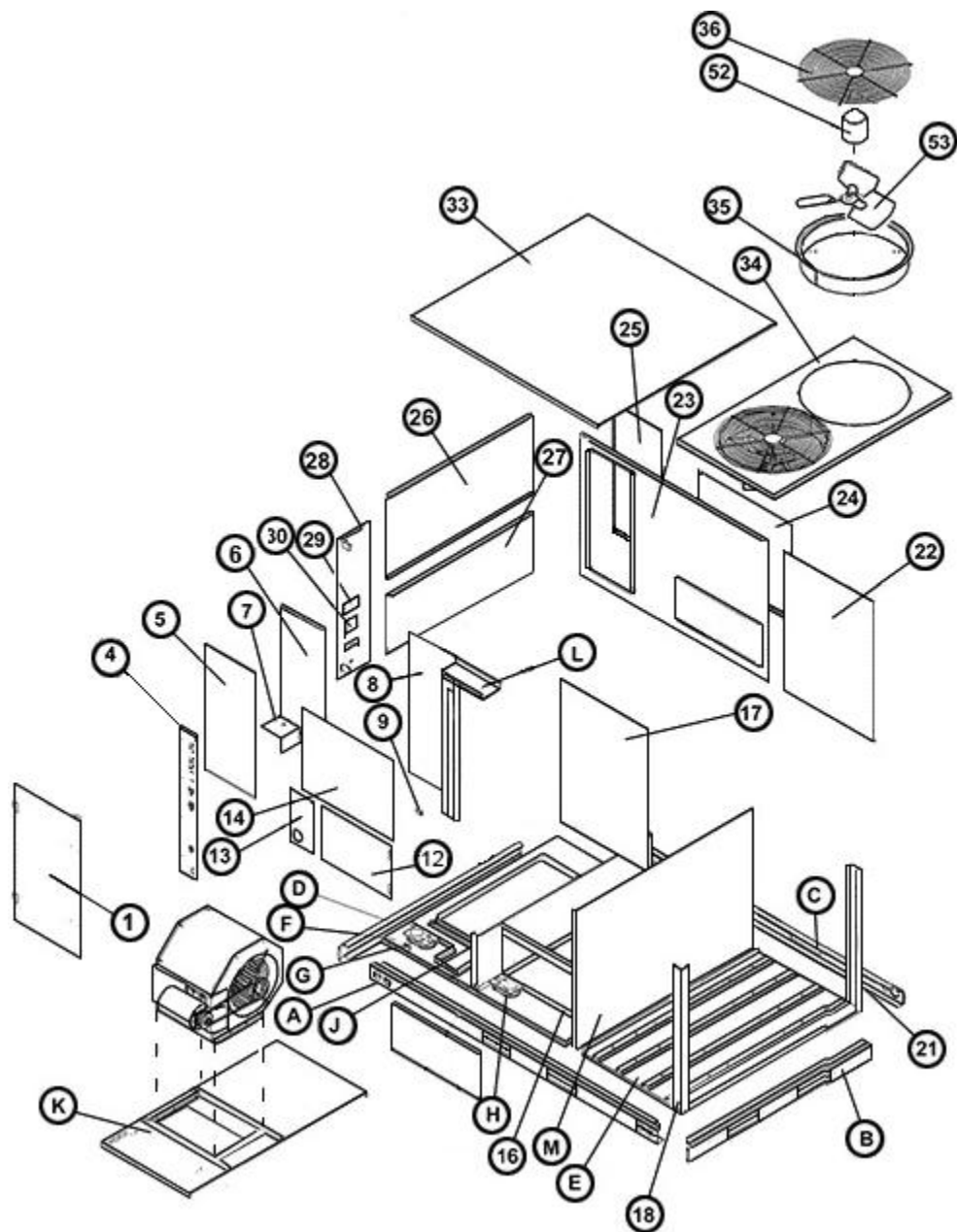
Exploded View 090-151
