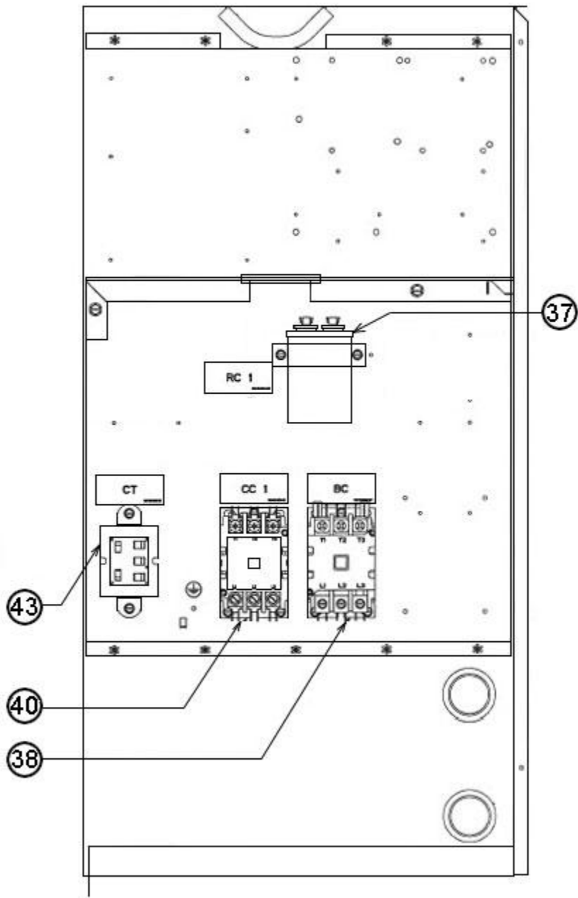
Control Box 072
