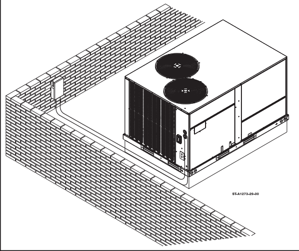
FIGURE 17 BRANCH CIRCUIT DISCONNECT LOCATION
