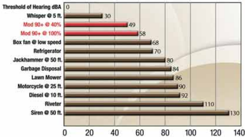
Sound Comparisons with the Rheem Prestige Series™ Modulating Gas Furnace
