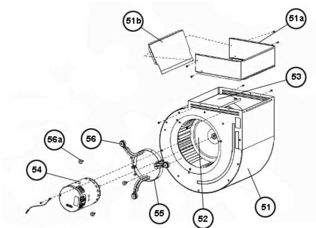
Blower Assembly
