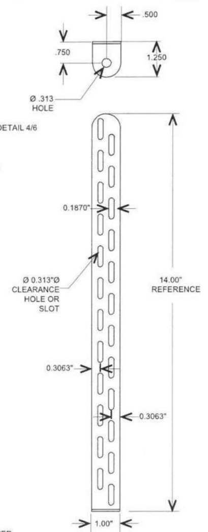
TIE-DOWN CLIP MIAMI TECH CLIP: 12GA (0.09") ASTM A653 Fu=90 KSI STEEL (CUTD14), MIAMI TECH KIT # RRCUTD34K
