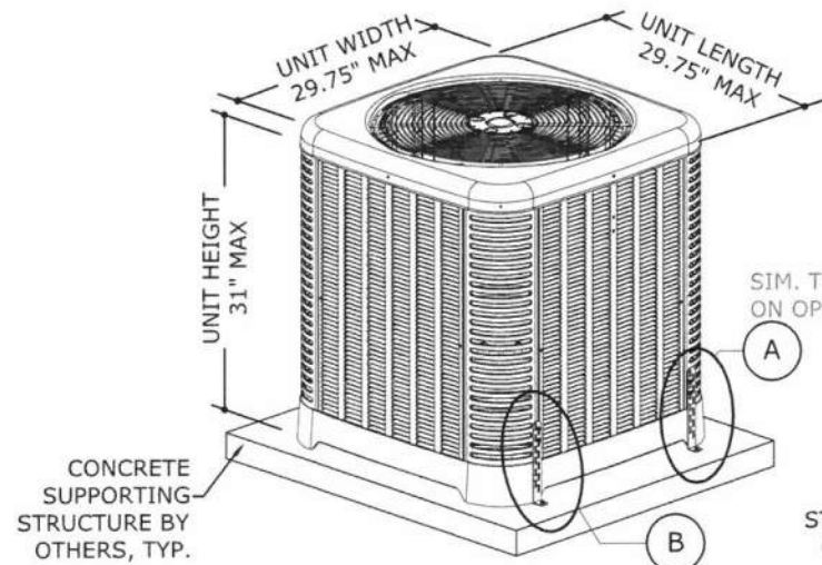
1 MECHANICAL UNIT 1 NOT TO SCALE FRONT ISOMETRIC
