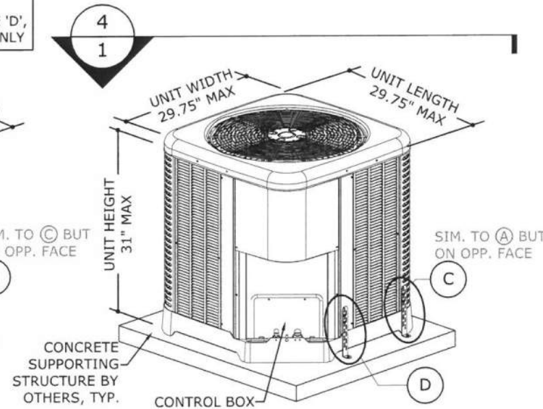
2 MECHANICAL UNIT 1 NOT TO SCALE BACK ISOMETRIC
