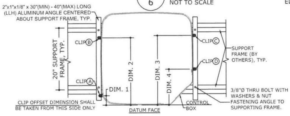
5 TIE-DOWN CLIP LAYOUT 6 NOT TO SCALE ELEVATIONS
