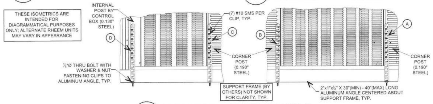
4 TIE-DOWN CLIP ATTACHMENTS 6 NOT TO SCALE ELEVATIONS
