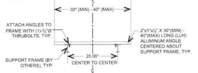
3 SUPPORT ANGLE 6 NOT TO SCALE ELEVATION
