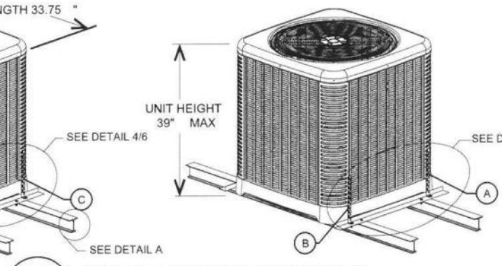
2 MOUNT ISOMETRIC VIEW 6 NOT TO SCALE FRONT ISO / BACK ISO
