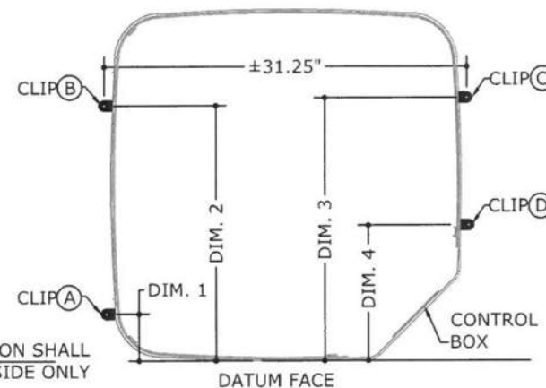
4 TIE-DOWN BRACKET LAYOUT 1 NOT TO SCALE PLAN
