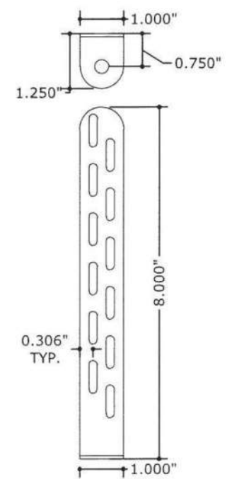
TIE-DOWN BRACKET MIAMI TECH CLIP: 14GA (0.07") ASTM A653 Fu=90 KSI STEEL (CUTD8) OR 0.080" 5052-H32 ALUMINUM (CUTDA8), MIAMI TECH KIT # RRCUTDSMK OR RRCUTDASMK
