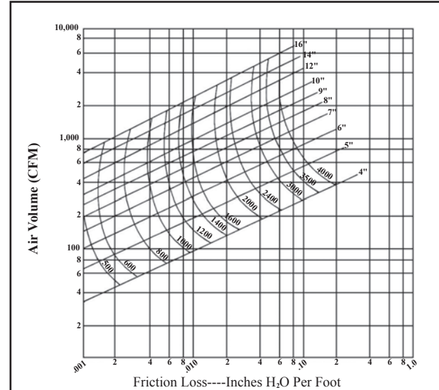
Friction Loss (ADC 72-R1) Straight Sections
