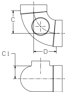
807-9 \Delta DWV 90° Elbow w/Side Inlet C x C x C – Cast
