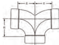
837 \Delta DWV 90° Double Elbow C x C x C – Cast
