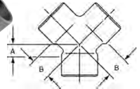
748 \Delta 90° Y C x C x C – Cast
