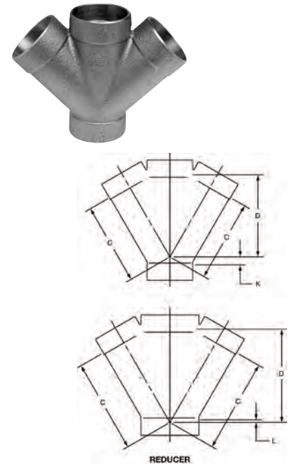
834 \Delta DWV 45° Double Y C x C x C x C – Cast
