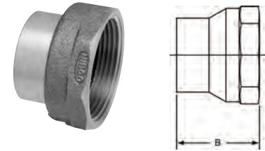
803-2 \Delta DWV Fitting Adapter Ftg x F – Cast
