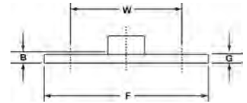
771 \Delta Threaded Companion Flange F – Cast
