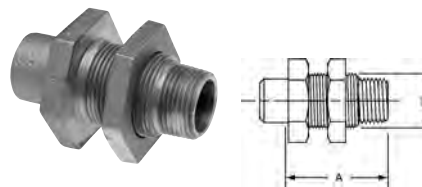
750-4 \Delta Bulkhead Fitting C x M – Cast
