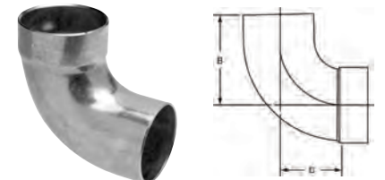
807-2 \Delta DWV 90° Fitting Elbow Ftg x C – Cast
