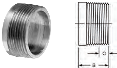
802-C \Delta DWV Flush Adapter C x M – Cast
