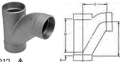
812 \Delta DWV Long Turn T-Y C x C x C – Cast
