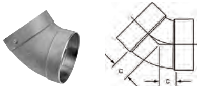
806 \Delta DWV 45° Elbow C x C – Cast
