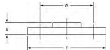
775 \Delta Threaded Companion Flange F – Cast
