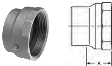
803 \Delta DWV Adapter C x F – Cast
