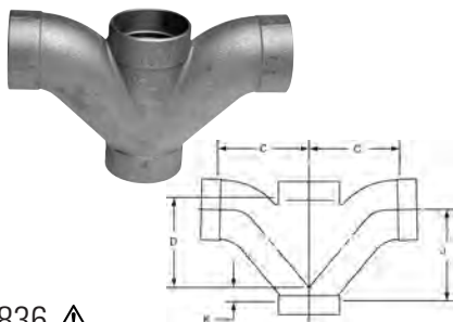
836 \Delta DWV Double Long Turn T-Y C x C x C x C – Cast
