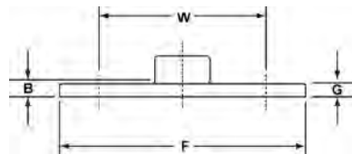
741 \Delta Companion Flange C – Cast
