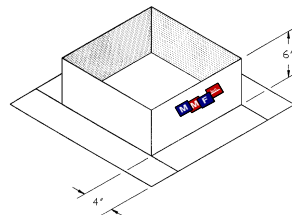
Cooler Flashing / Flat Page 20C - 20CC
