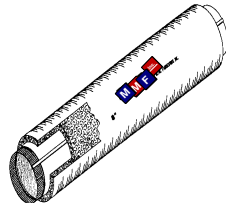
Button-lock Pipe Page 6A
