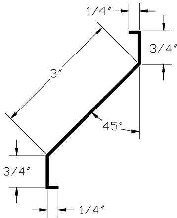
Blade Detail
