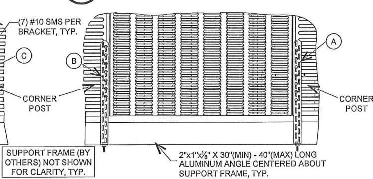
4 TIE-DOWN BRACKET ATTACHMENTS 1 N.T.S. ELEVATIONS
