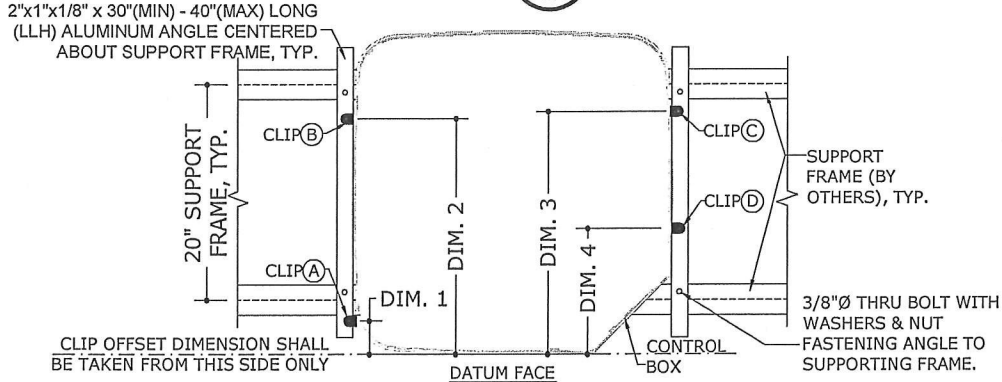
5 TIE-DOWN BRACKET LAYOUT 1 N.T.S. PLAN
