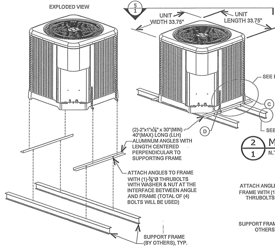
1 MOUNT EXPLODED VIEW 1 N.T.S. FRONT ISOMETRIC
