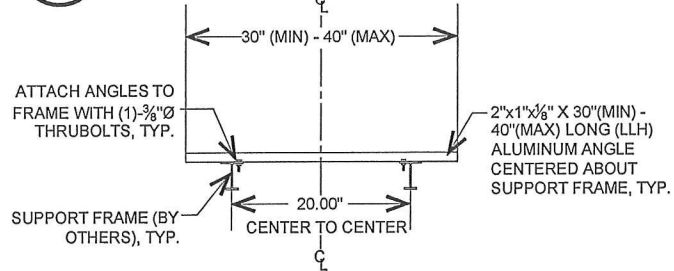
3 SUPPORT ANGLE 1 N.T.S. ELEVATION
