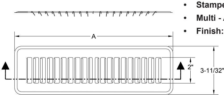
Toe Space Grille Dimensional Chart
