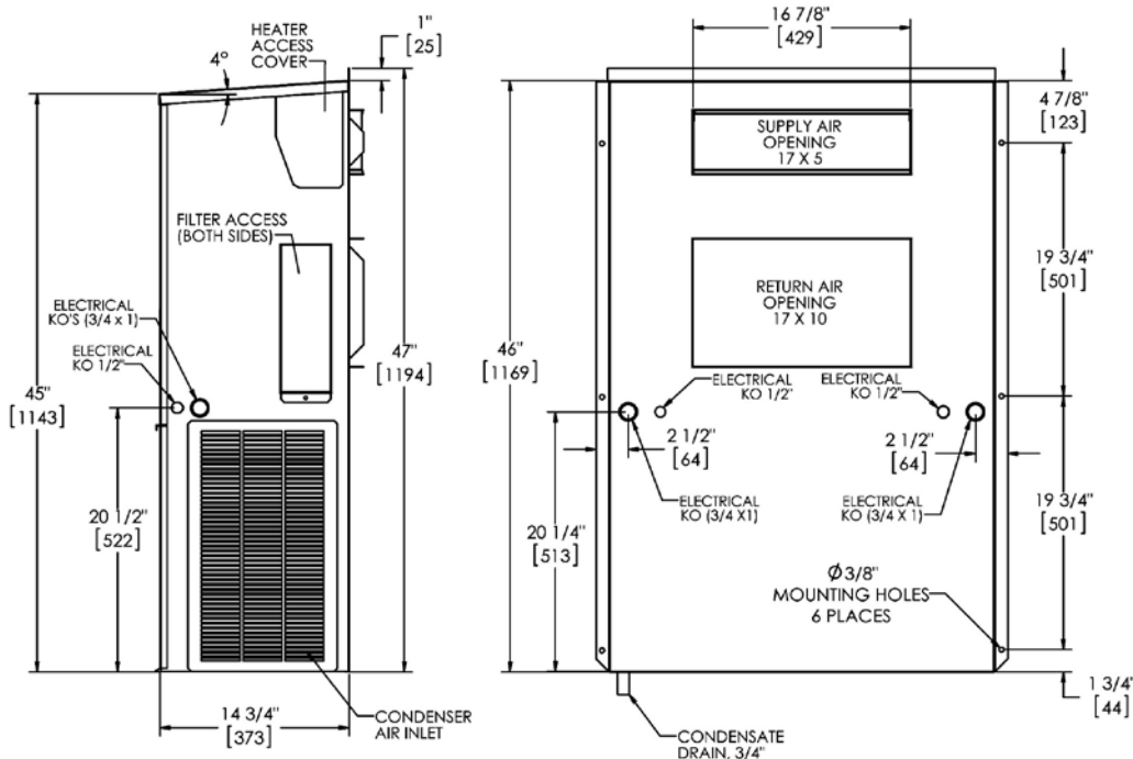
RH SIDE VIEW
