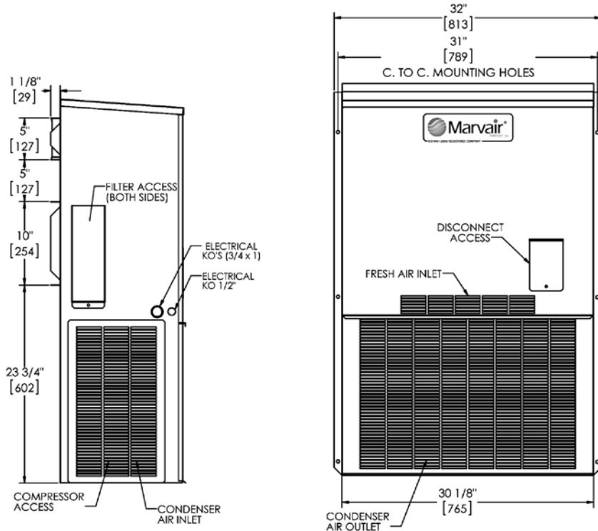
LH SIDE VIEW
