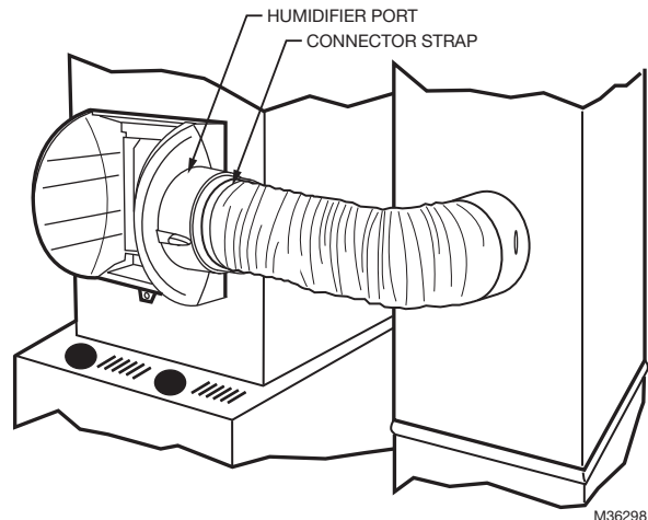
Fig. 6. Connecting bypass ducting.
