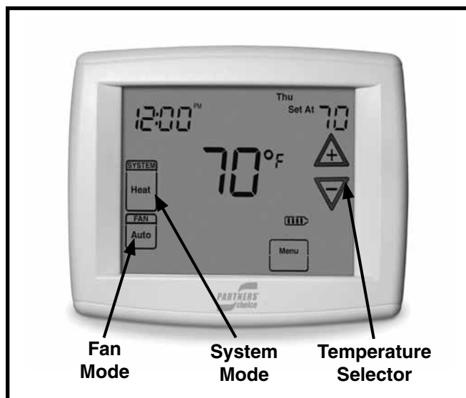
Figure 1. Digital Thermostat
