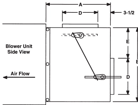
Mixing Box Side View
