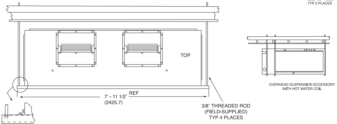
UNIT SIZES 150-240 (FRONT)
