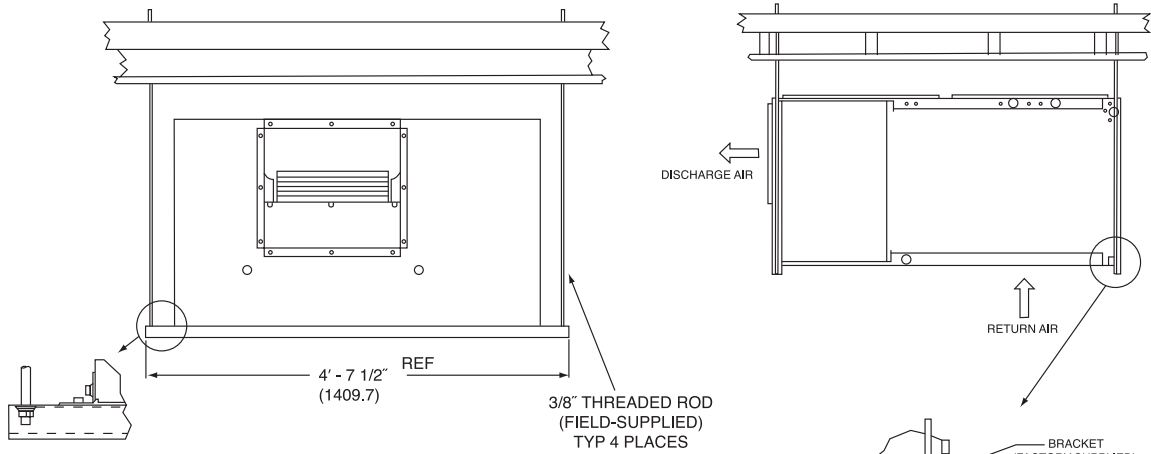
UNIT SIZES 150-240 (FRONT)
