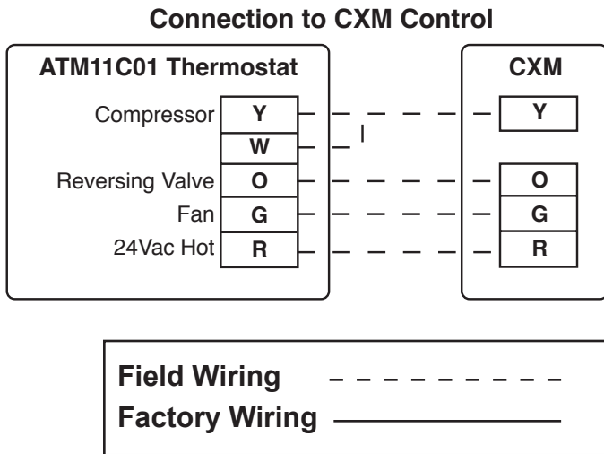
Figure 22: Units With PSC Fan And CXM
