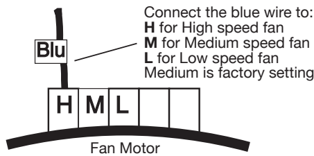
Figure 16: PSC Motor Speed Selection
