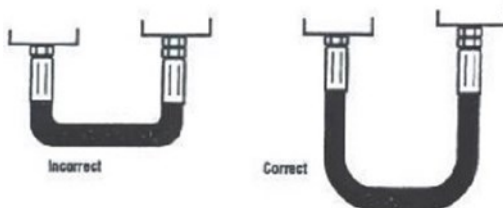
FIGURE 1 — HOSE AND MACHINE TOLERANCES
