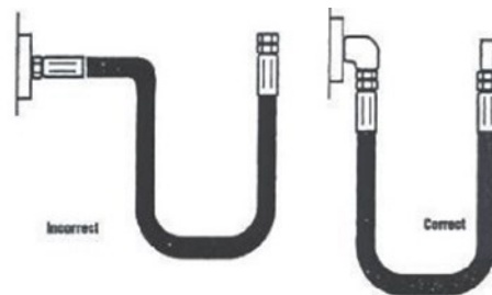
FIGURE 2 — ELBOWS AND ADAPTERS
