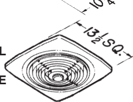
MODEL 505 GRILLE
