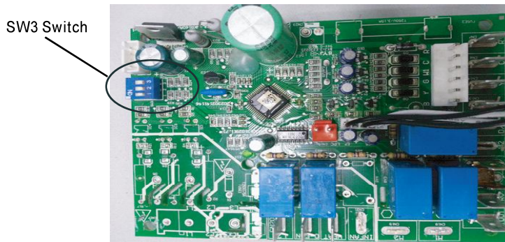
Fig.11 SW3 Switch Location in the PCB Board
