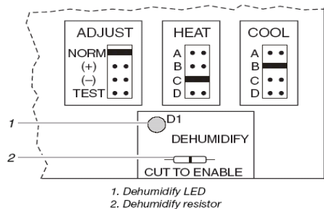
Control Board Taps and Dehumidify Resistor.
